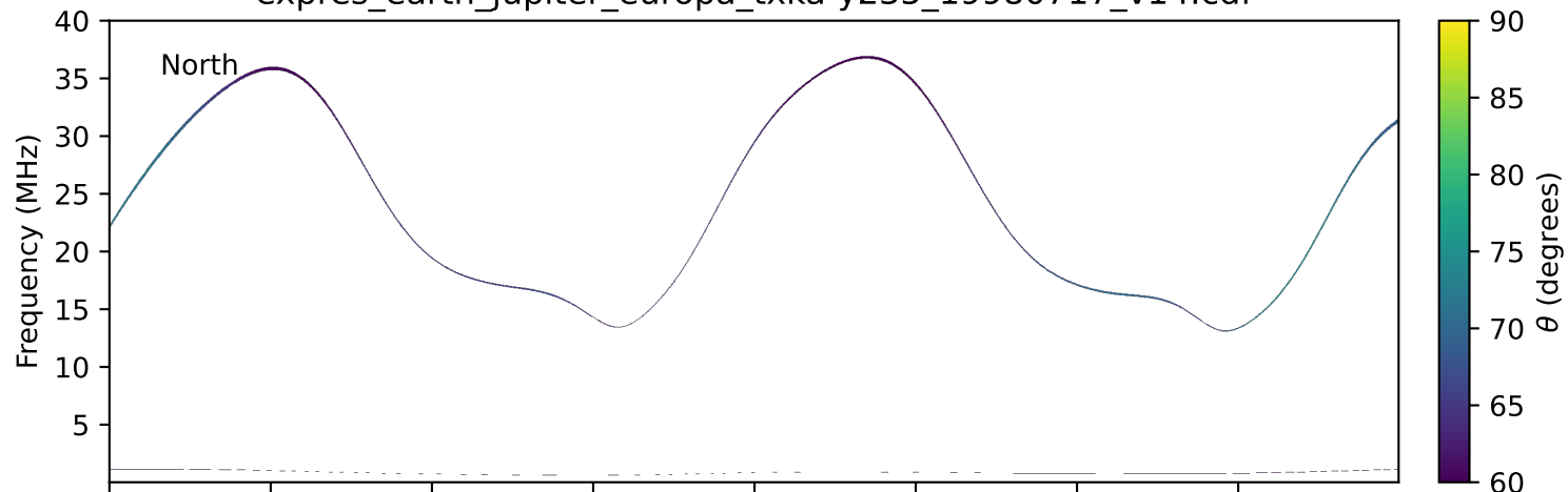
expres_earth_jupiter_europa_txka-y235_19980717_v14.cdf
