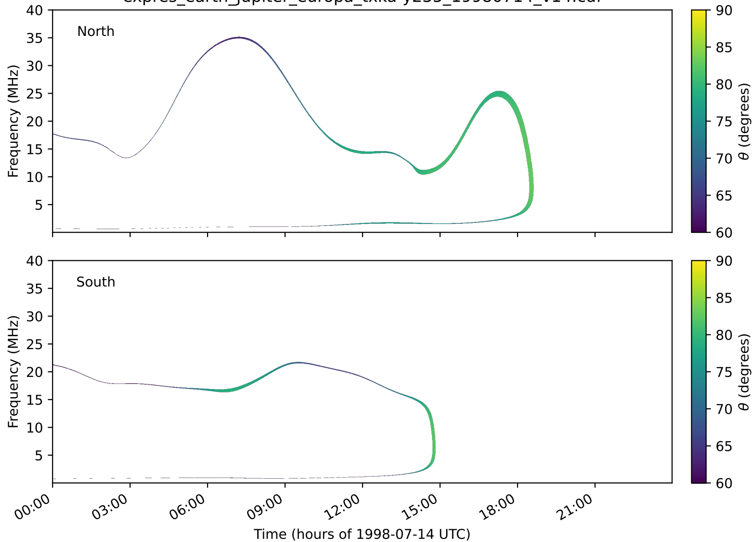
expres_earth_jupiter_europa_txka-y235_19980714_v14.cdf
