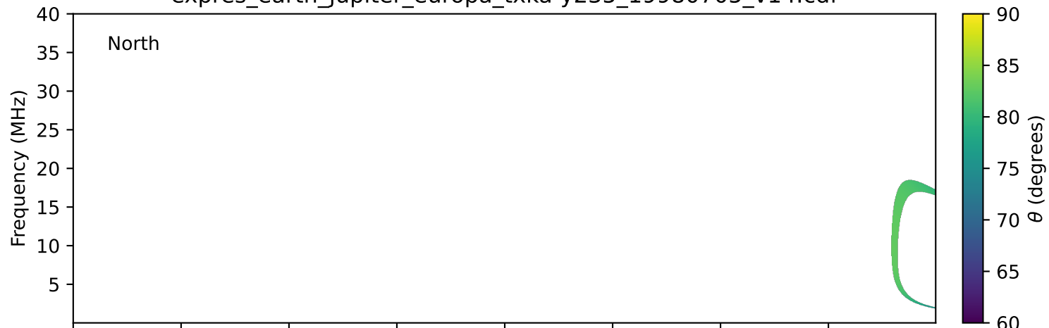
expres_earth_jupiter_europa_txka-y235_19980705_v14.cdf
