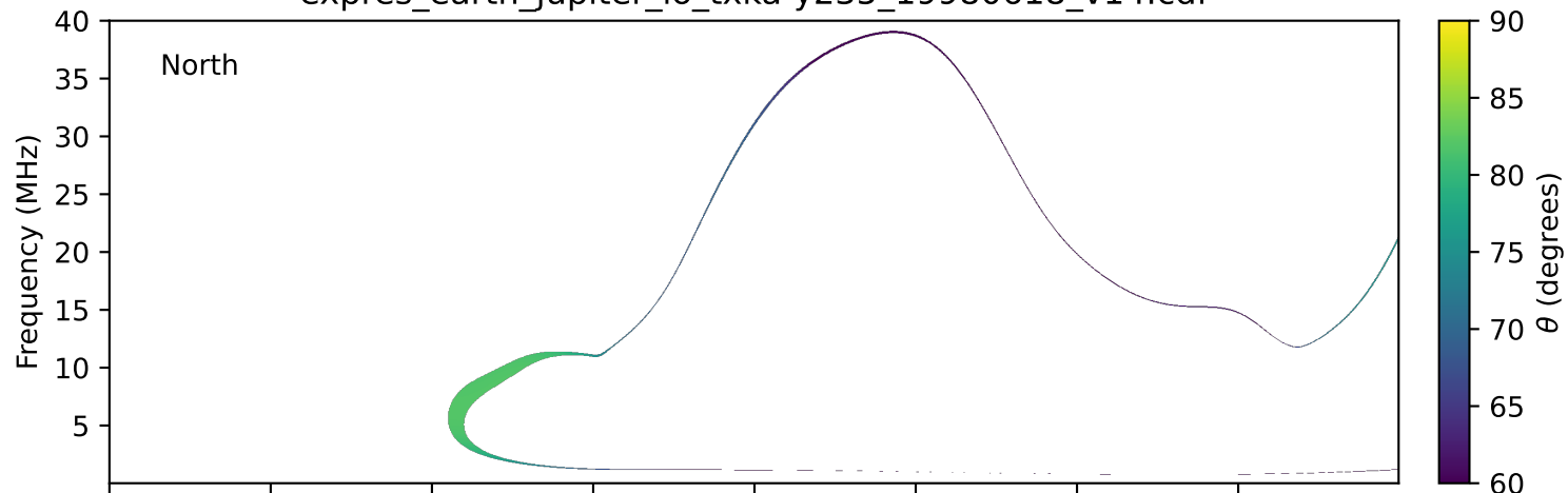
expres_earth_jupiter_io_txka-y235_19980618_v14.cdf
