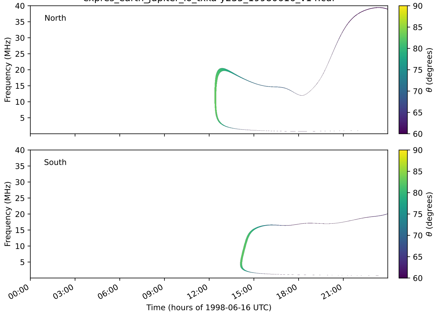
expres_earth_jupiter_io_txka-y235_19980616_v14.cdf
