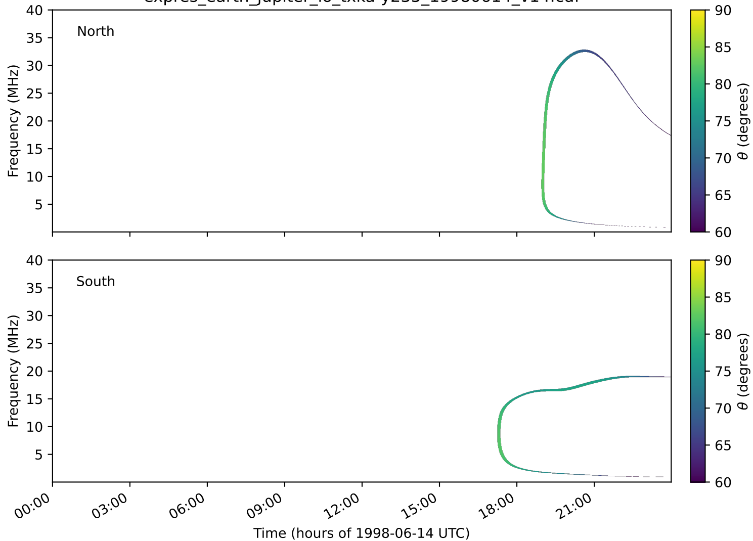
expres_earth_jupiter_io_txka-y235_19980614_v14.cdf
