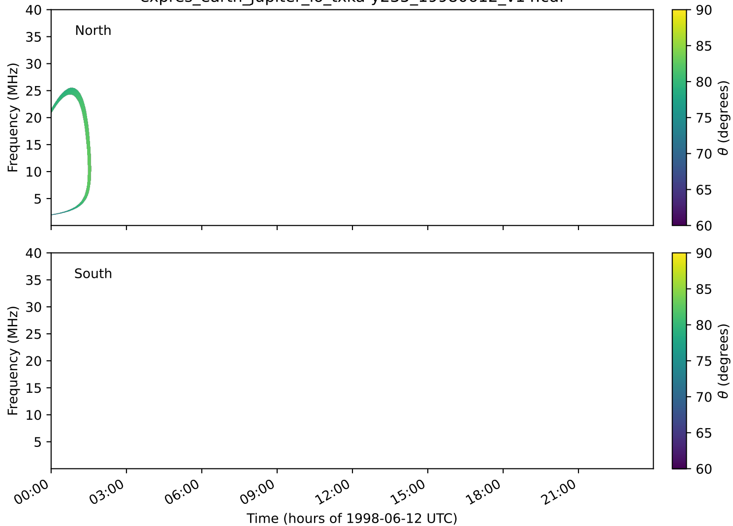
expres_earth_jupiter_io_txka-y235_19980612_v14.cdf
