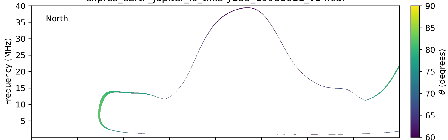
expres_earth_jupiter_io_txka-y235_19980611_v14.cdf
