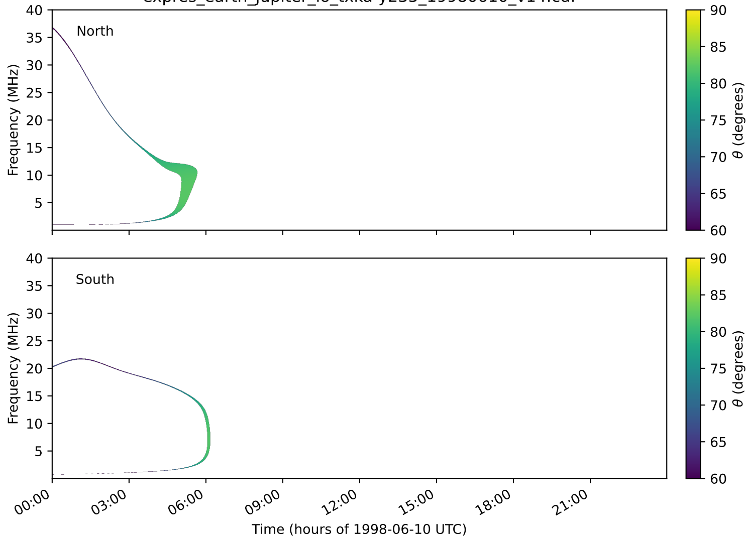
expres_earth_jupiter_io_txka-y235_19980610_v14.cdf
