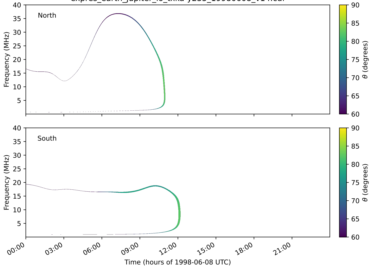
expres_earth_jupiter_io_txka-y235_19980608_v14.cdf
