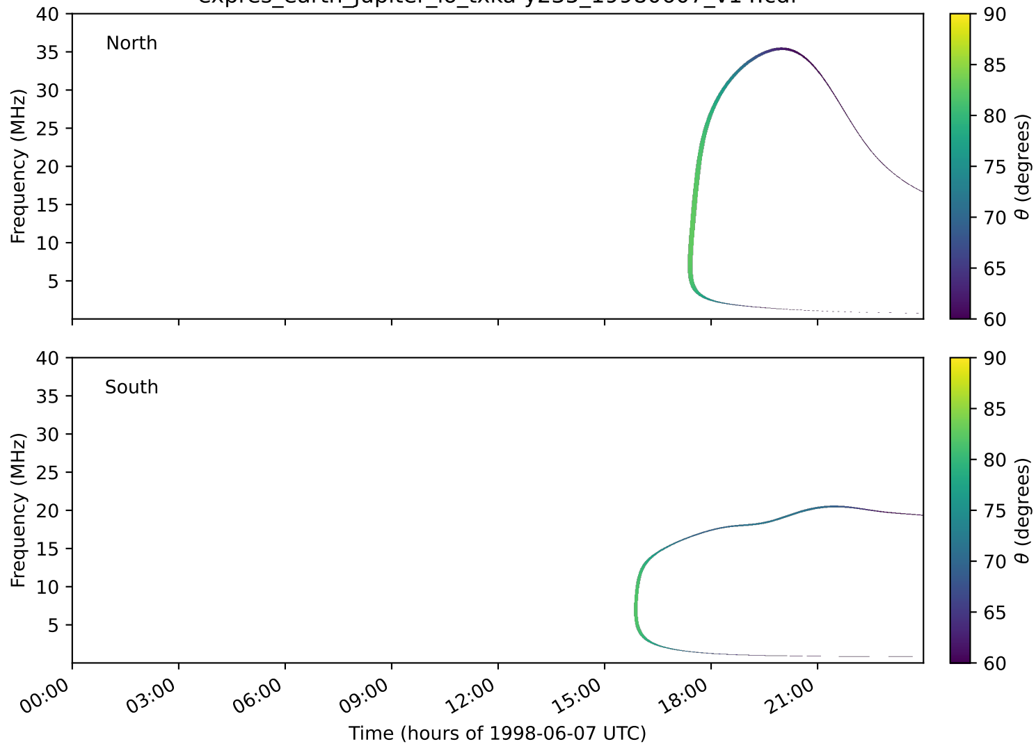
expres_earth_jupiter_io_txka-y235_19980607_v14.cdf
