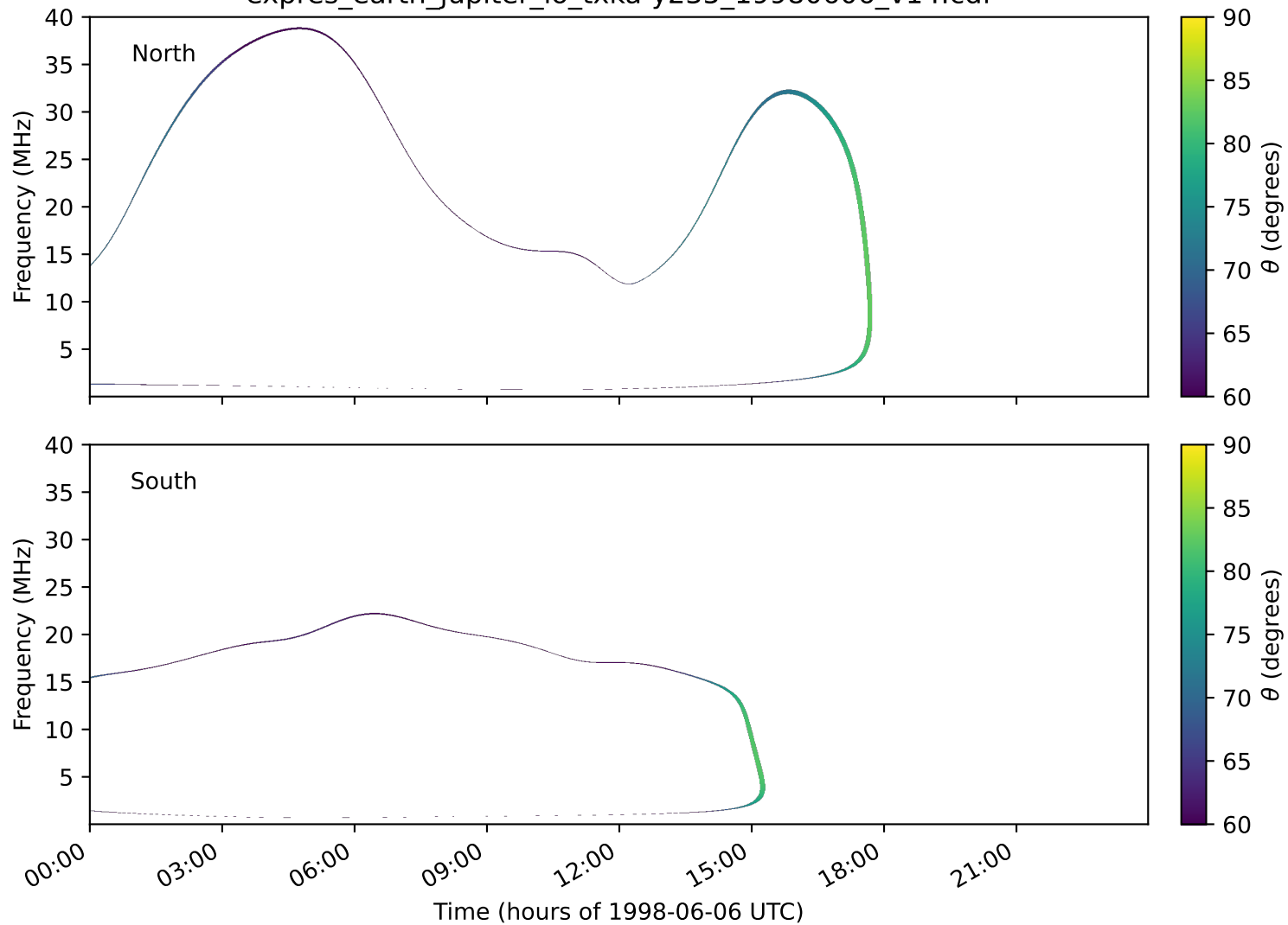
expres_earth_jupiter_io_txka-y235_19980606_v14.cdf
