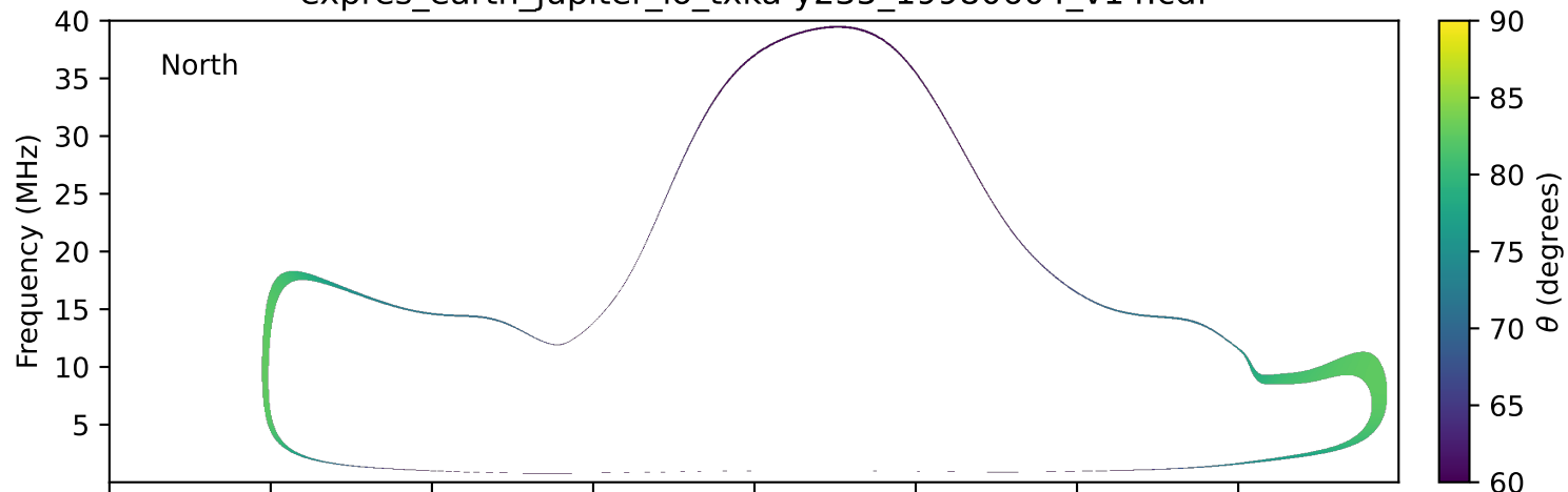
expres_earth_jupiter_io_txka-y235_19980604_v14.cdf
