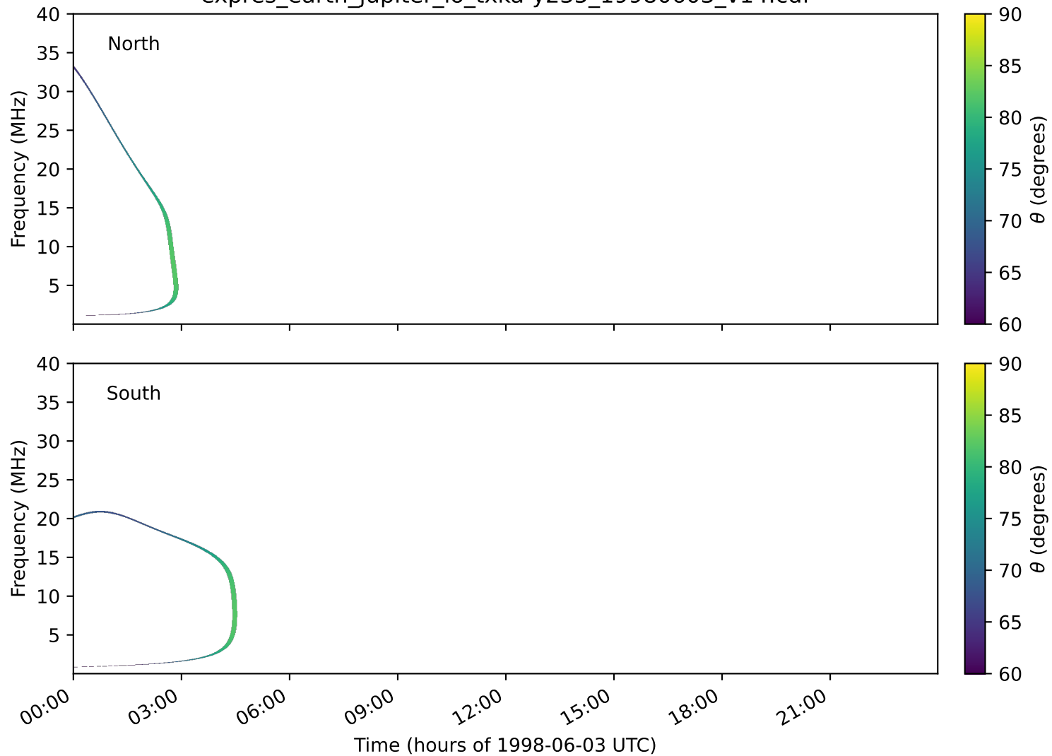
expres_earth_jupiter_io_txka-y235_19980603_v14.cdf
