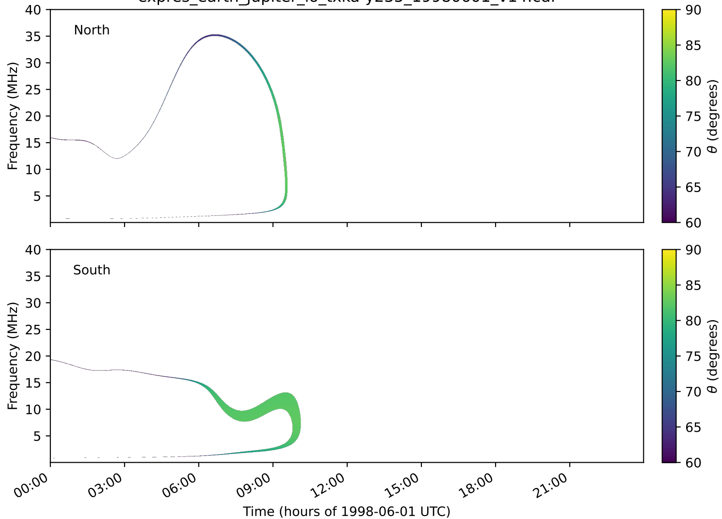
expres_earth_jupiter_io_txka-y235_19980601_v14.cdf
