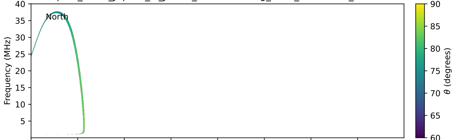
expres_earth_jupiter_io_jrm33_lossc-wid1deg_3kev_19980619_v11.cdf
