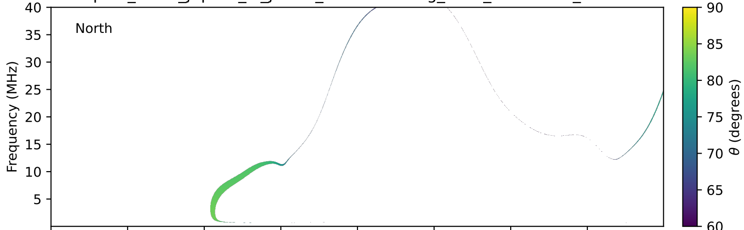
expres_earth_jupiter_io_jrm33_lossc-wid1deg_3kev_19980618_v11.cdf
