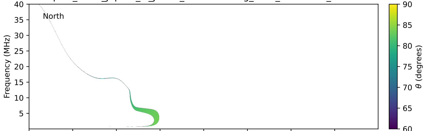
expres_earth_jupiter_io_jrm33_lossc-wid1deg_3kev_19980617_v11.cdf
