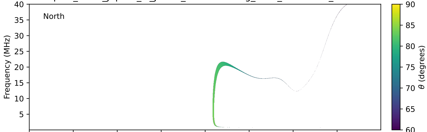
expres_earth_jupiter_io_jrm33_lossc-wid1deg_3kev_19980616_v11.cdf
