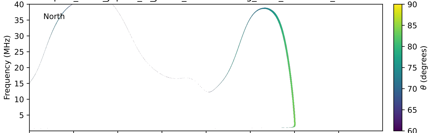
expres_earth_jupiter_io_jrm33_lossc-wid1deg_3kev_19980606_v11.cdf
