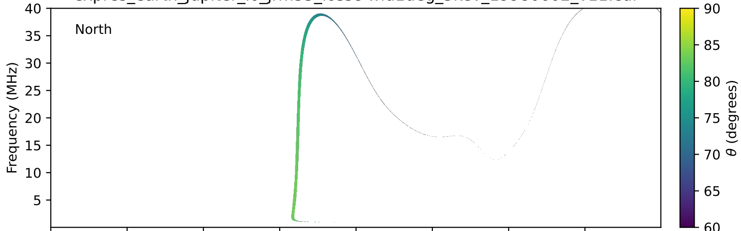
expres_earth_jupiter_io_jrm33_lossc-wid1deg_3kev_19980602_v11.cdf
