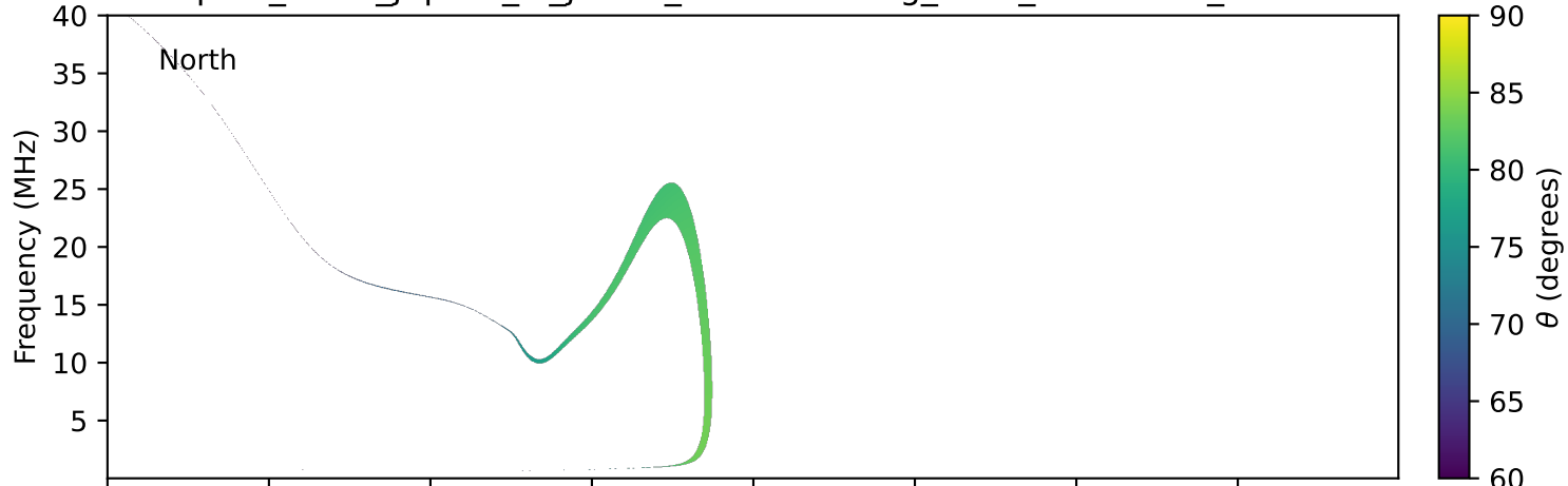
expres_earth_jupiter_io_jrm09_lossc-wid1deg_3kev_19980624_v11.cdf
