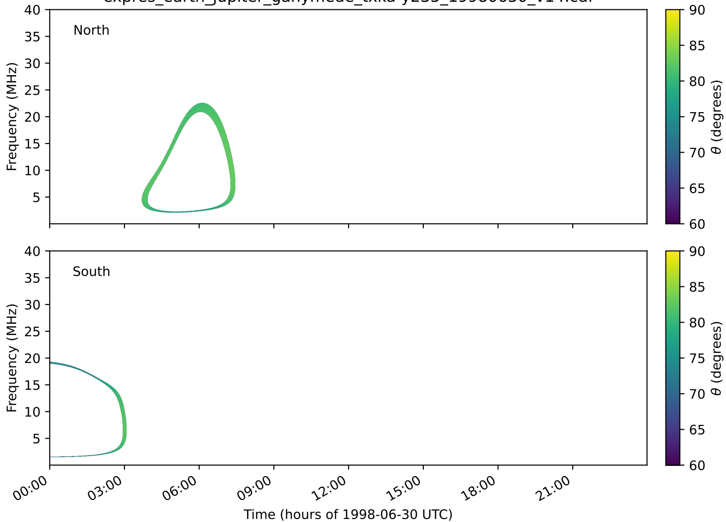
expres_earth_jupiter_ganymede_txka-y235_19980630_v14.cdf
