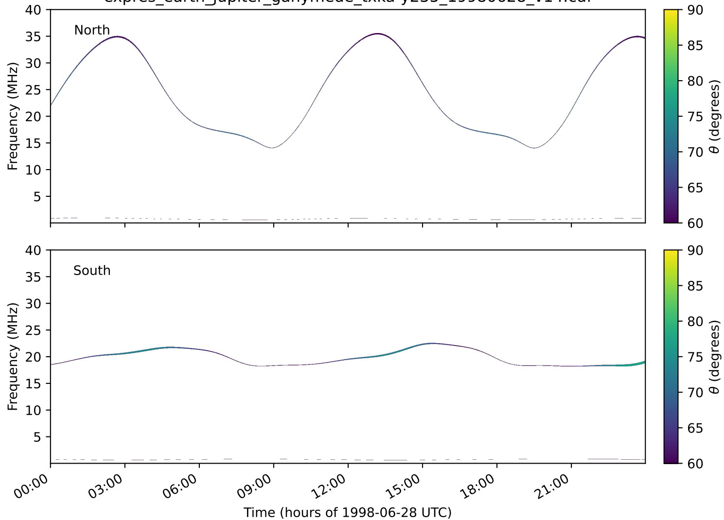
expres_earth_jupiter_ganymede_txka-y235_19980628_v14.cdf
