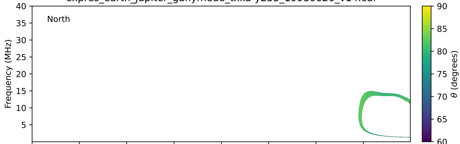
expres_earth_jupiter_ganymede_txka-y235_19980626_v14.cdf
