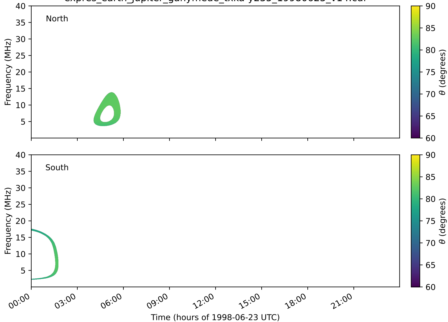
expres_earth_jupiter_ganymede_txka-y235_19980623_v14.cdf
