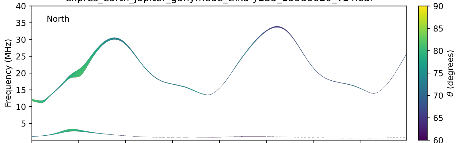
expres_earth_jupiter_ganymede_txka-y235_19980620_v14.cdf
