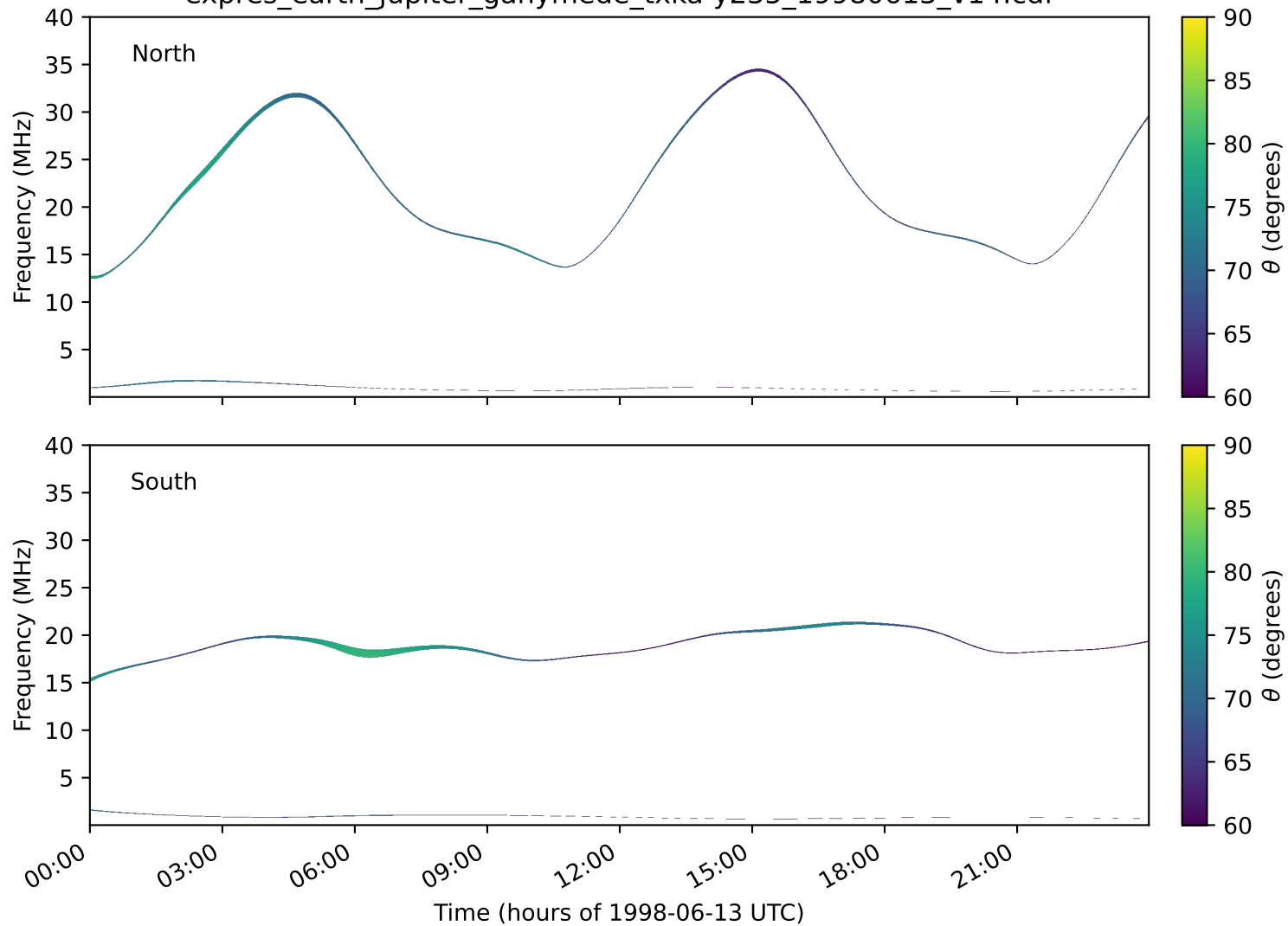
expres_earth_jupiter_ganymede_txka-y235_19980613_v14.cdf
