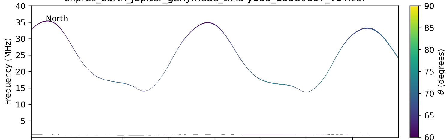
expres_earth_jupiter_ganymede_txka-y235_19980607_v14.cdf
