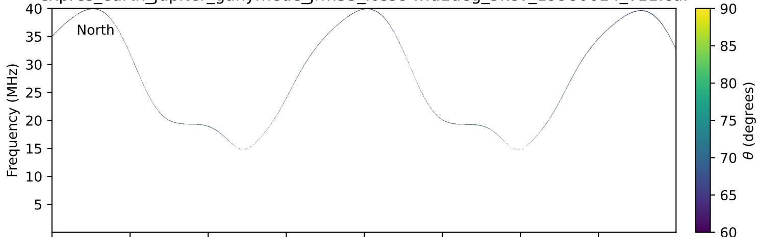
expres_earth_jupiter_ganymede_jrm33_lossc-wid1deg_3kev_19980614_v11.cdf
