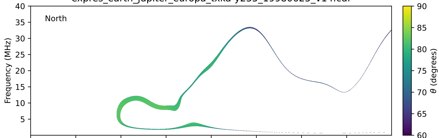
expres_earth_jupiter_europa_txka-y235_19980625_v14.cdf
