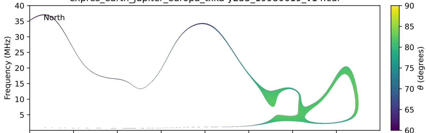
expres_earth_jupiter_europa_txka-y235_19980619_v14.cdf
