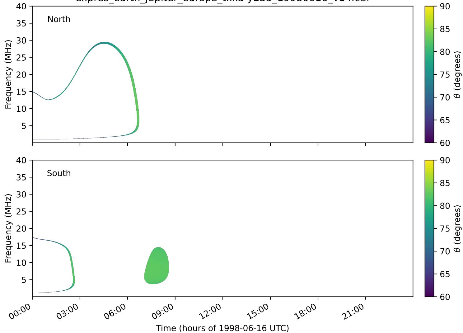
expres_earth_jupiter_europa_txka-y235_19980616_v14.cdf
