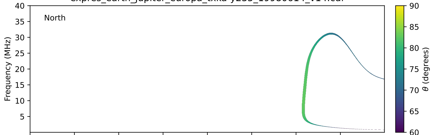
expres_earth_jupiter_europa_txka-y235_19980614_v14.cdf
