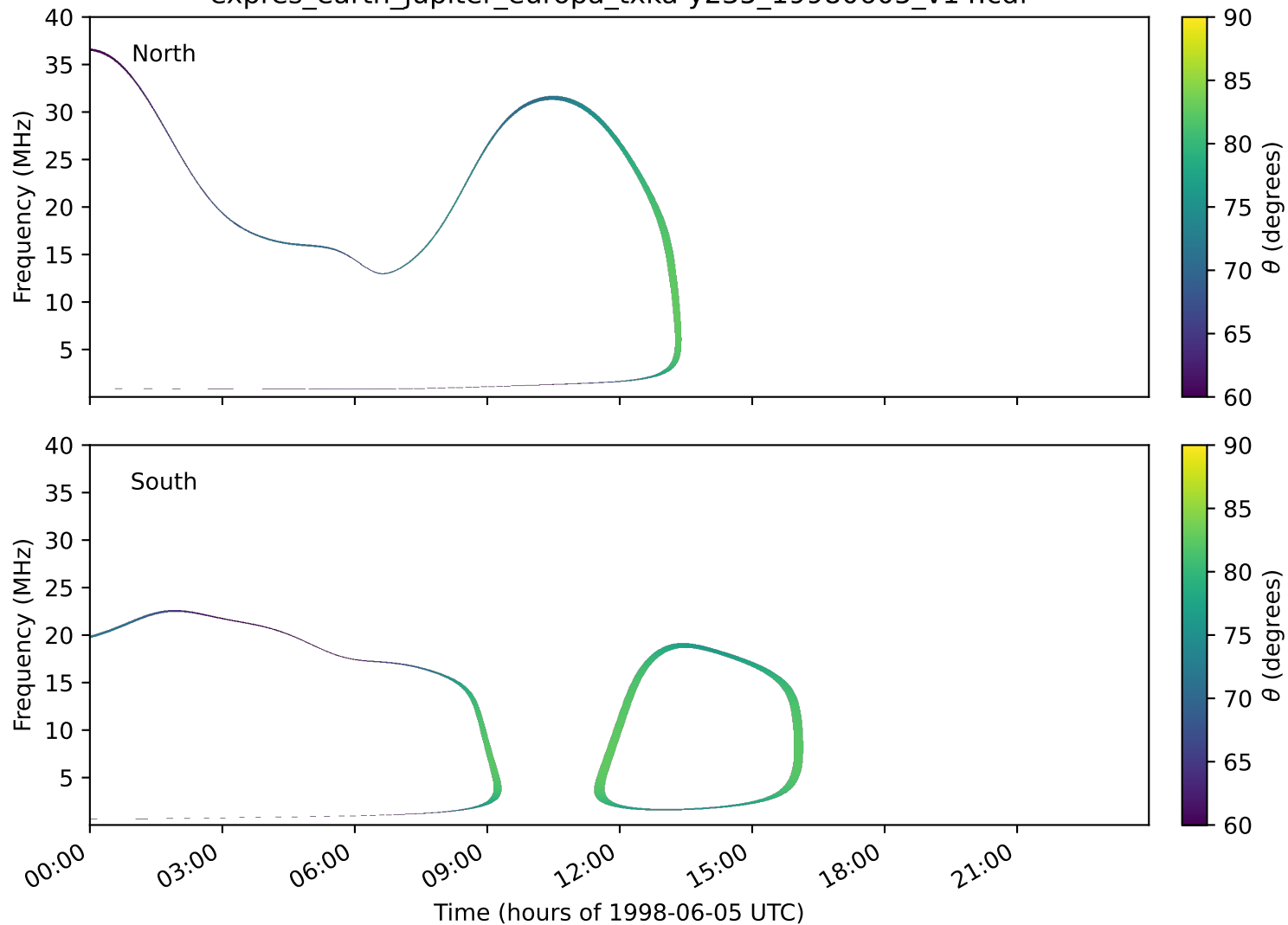
expres_earth_jupiter_europa_txka-y235_19980605_v14.cdf
