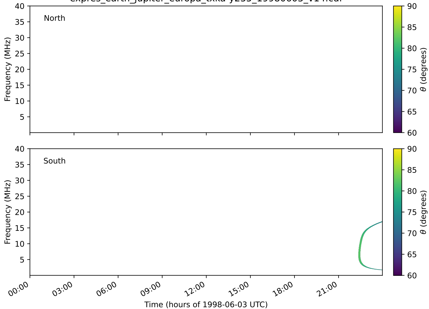
expres_earth_jupiter_europa_txka-y235_19980603_v14.cdf
