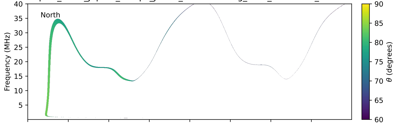
expres_earth_jupiter_europa_jrm33_lossc-wid1deg_3kev_19980604_v11.cdf
