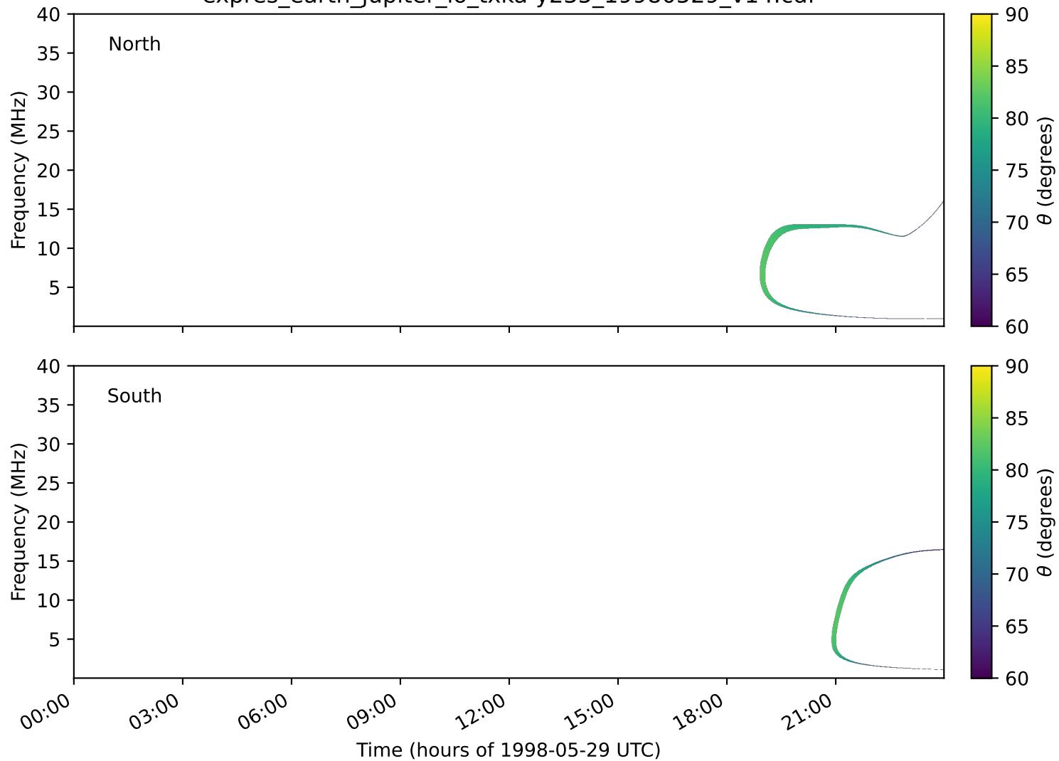
expres_earth_jupiter_io_txka-y235_19980529_v14.cdf
