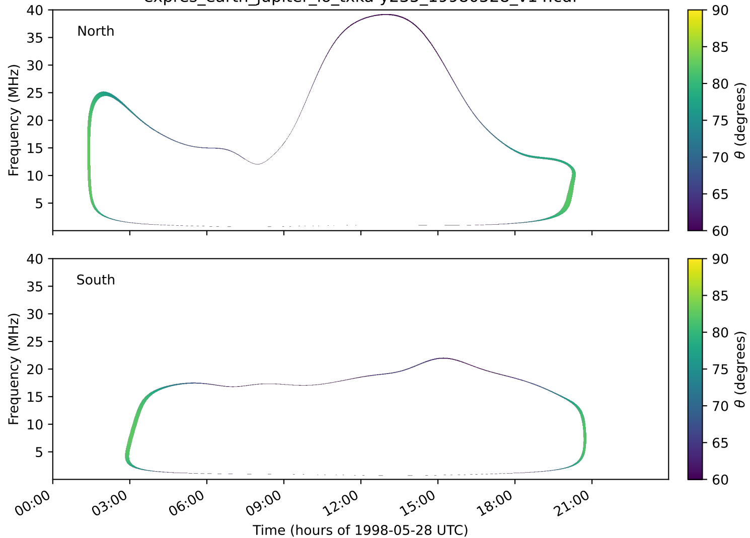
expres_earth_jupiter_io_txka-y235_19980528_v14.cdf
