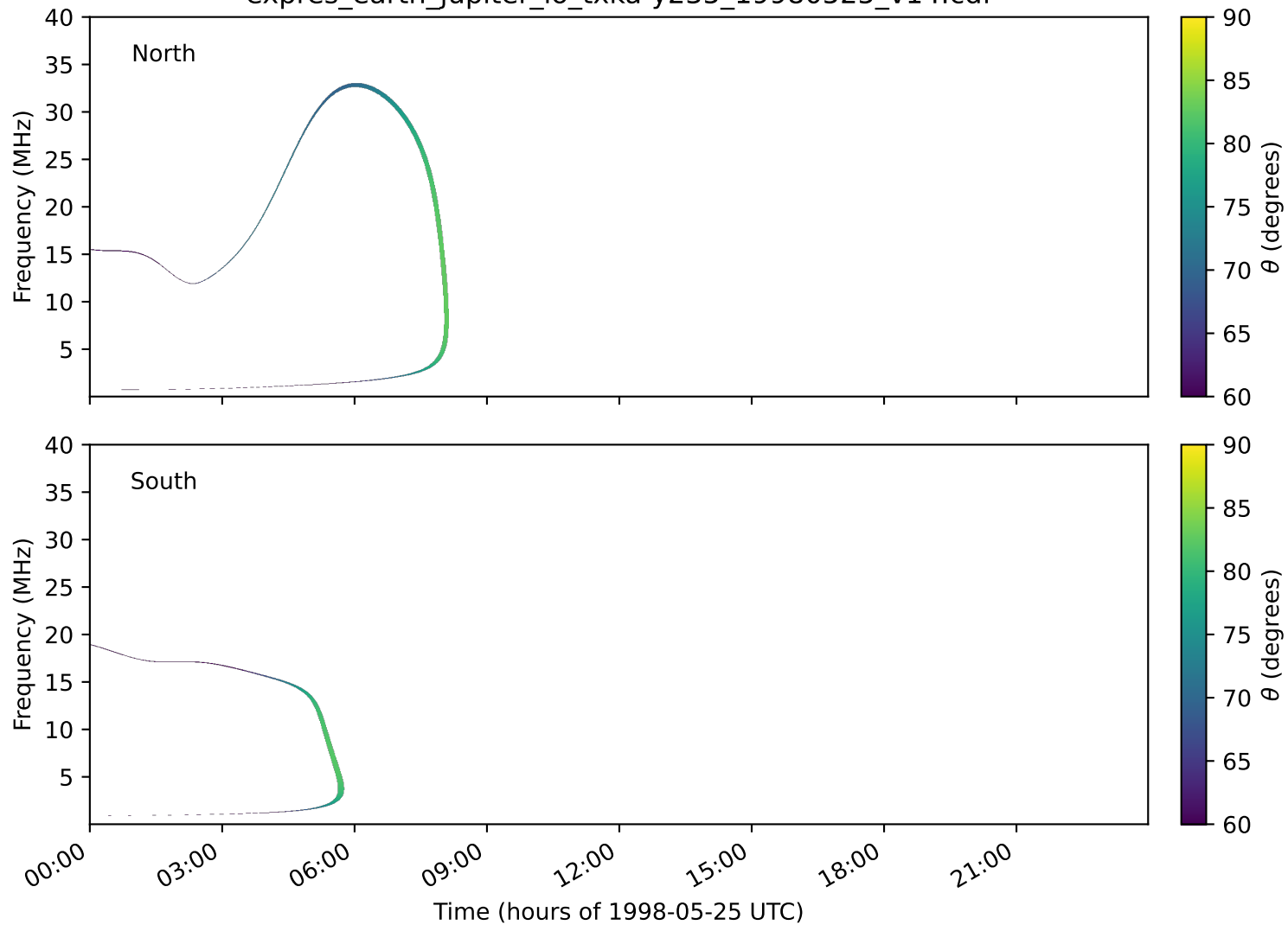
expres_earth_jupiter_io_txka-y235_19980525_v14.cdf
