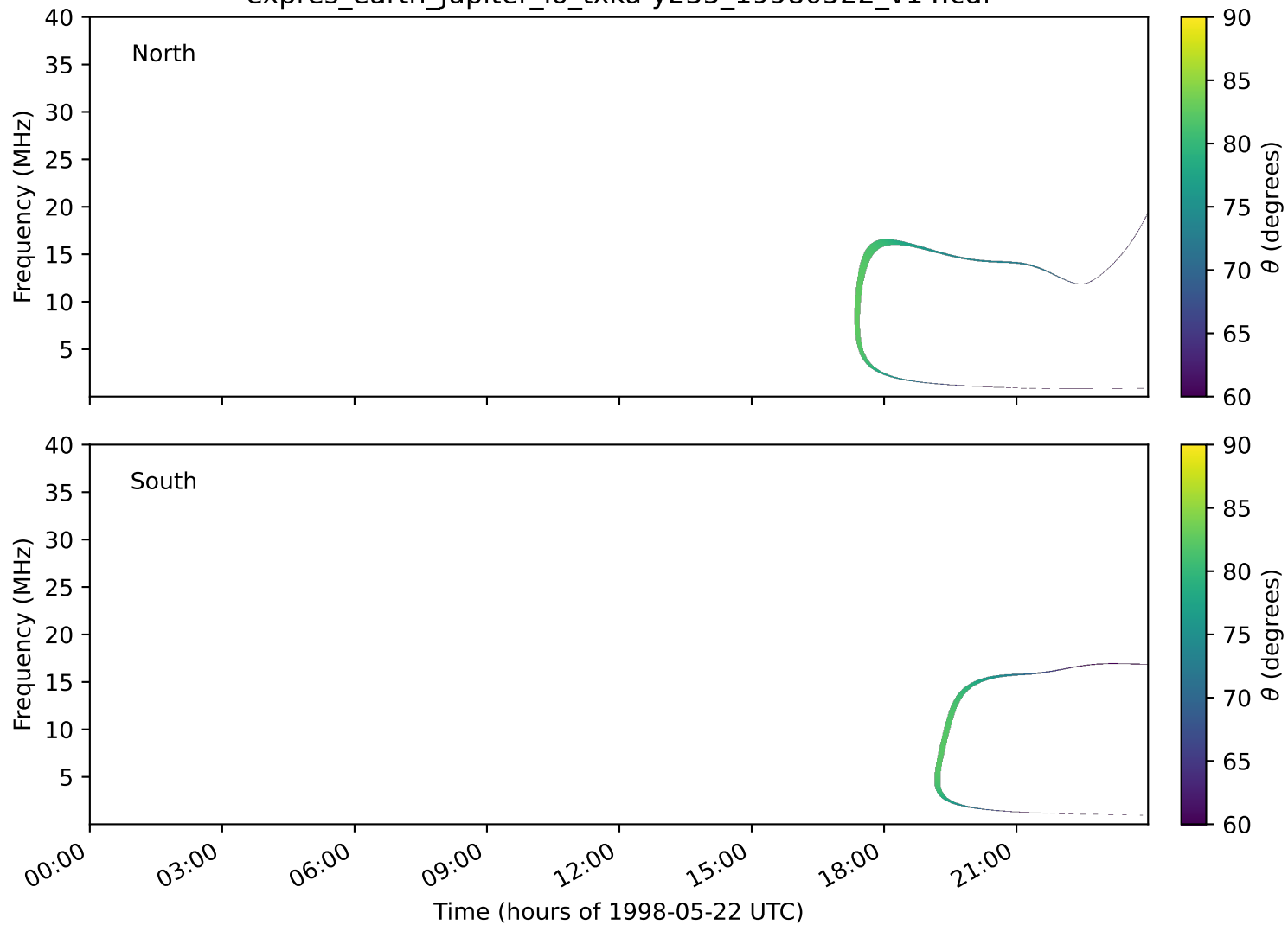
expres_earth_jupiter_io_txka-y235_19980522_v14.cdf
