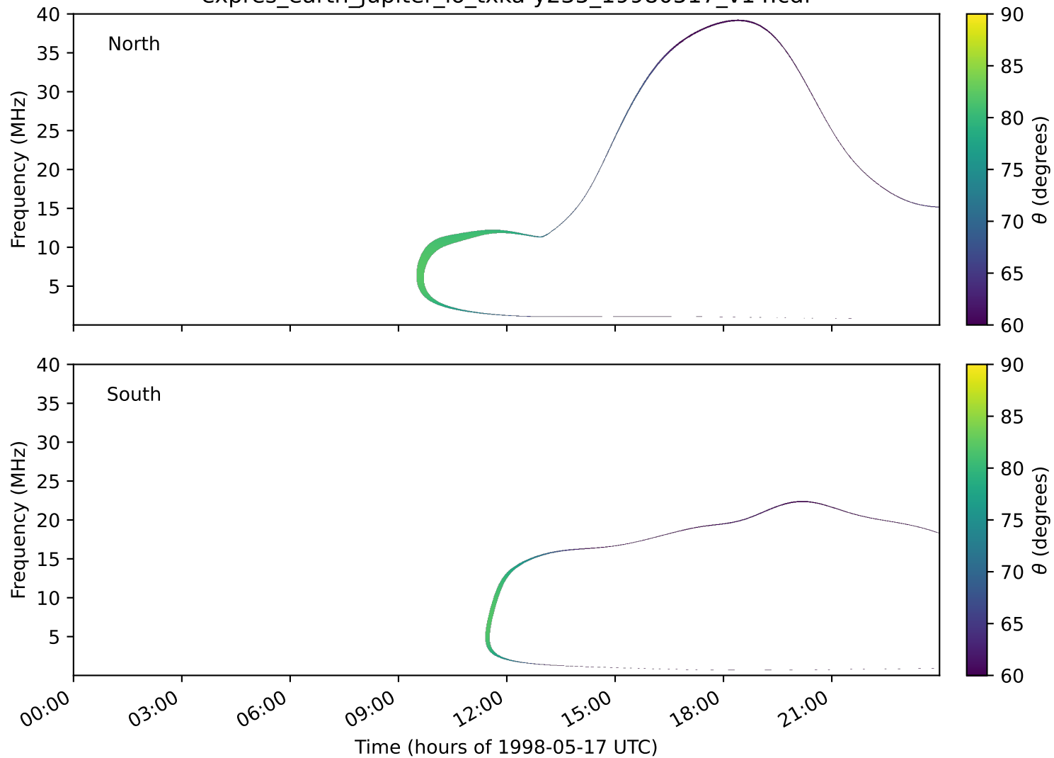
expres_earth_jupiter_io_txka-y235_19980517_v14.cdf
