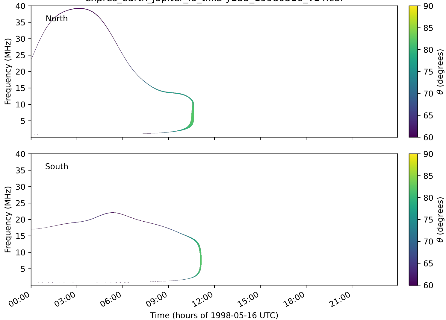
expres_earth_jupiter_io_txka-y235_19980516_v14.cdf
