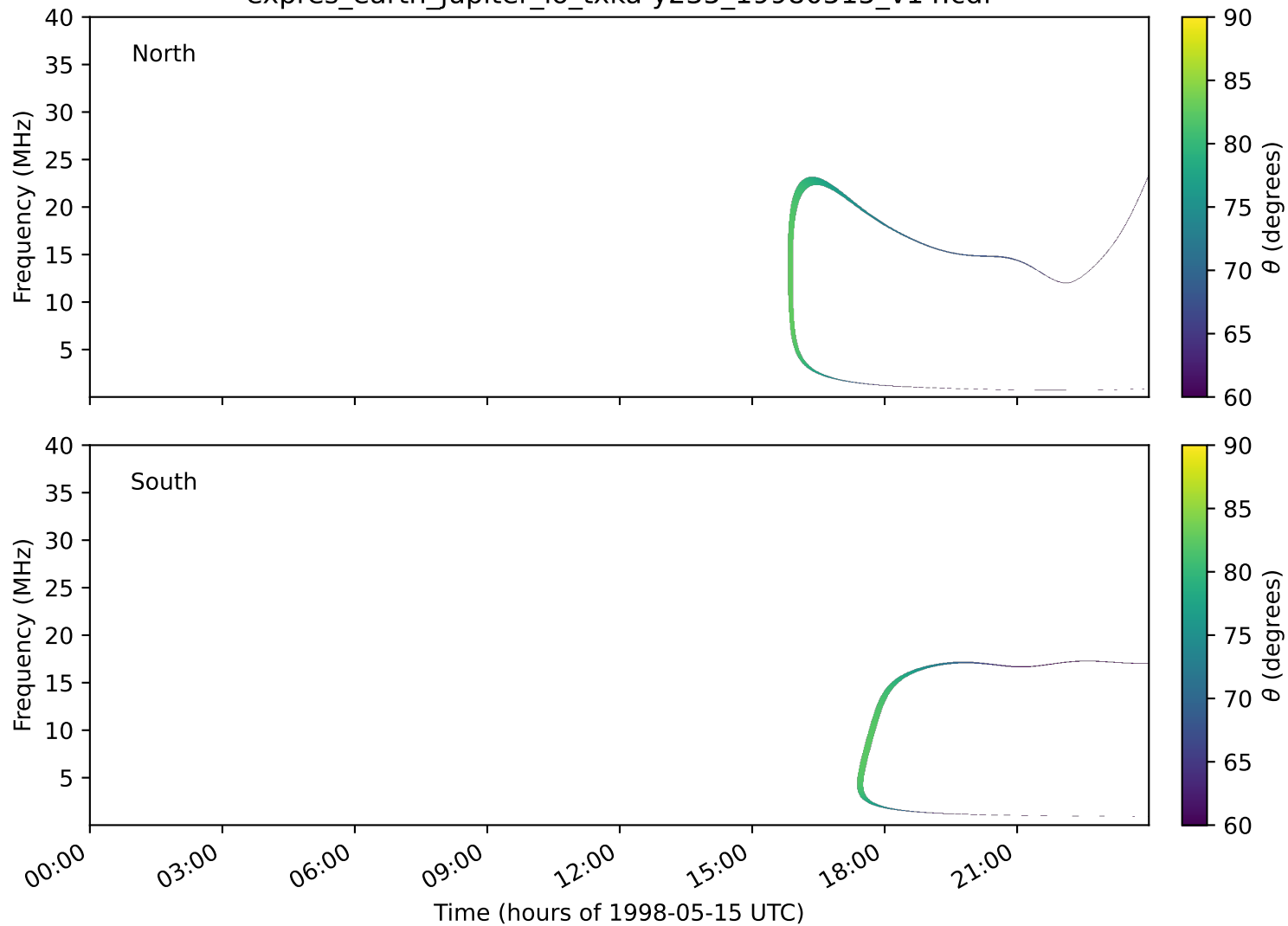
expres_earth_jupiter_io_txka-y235_19980515_v14.cdf
