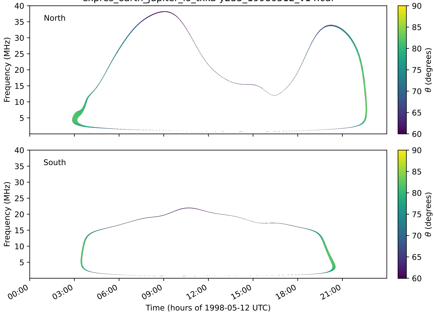
expres_earth_jupiter_io_txka-y235_19980512_v14.cdf
