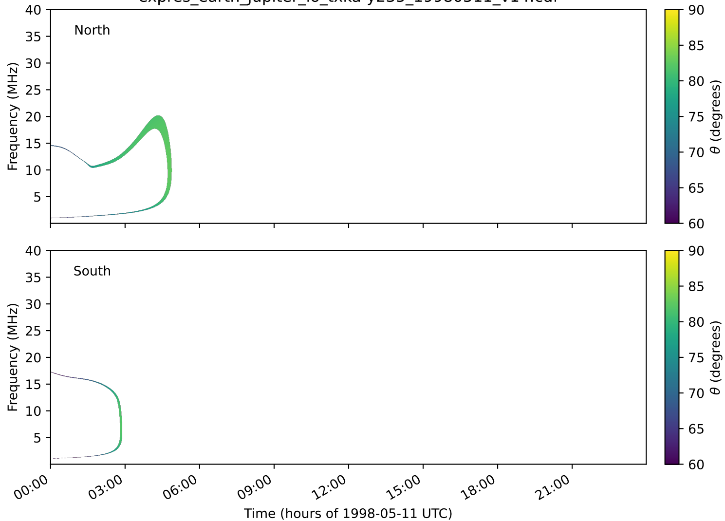
expres_earth_jupiter_io_txka-y235_19980511_v14.cdf
