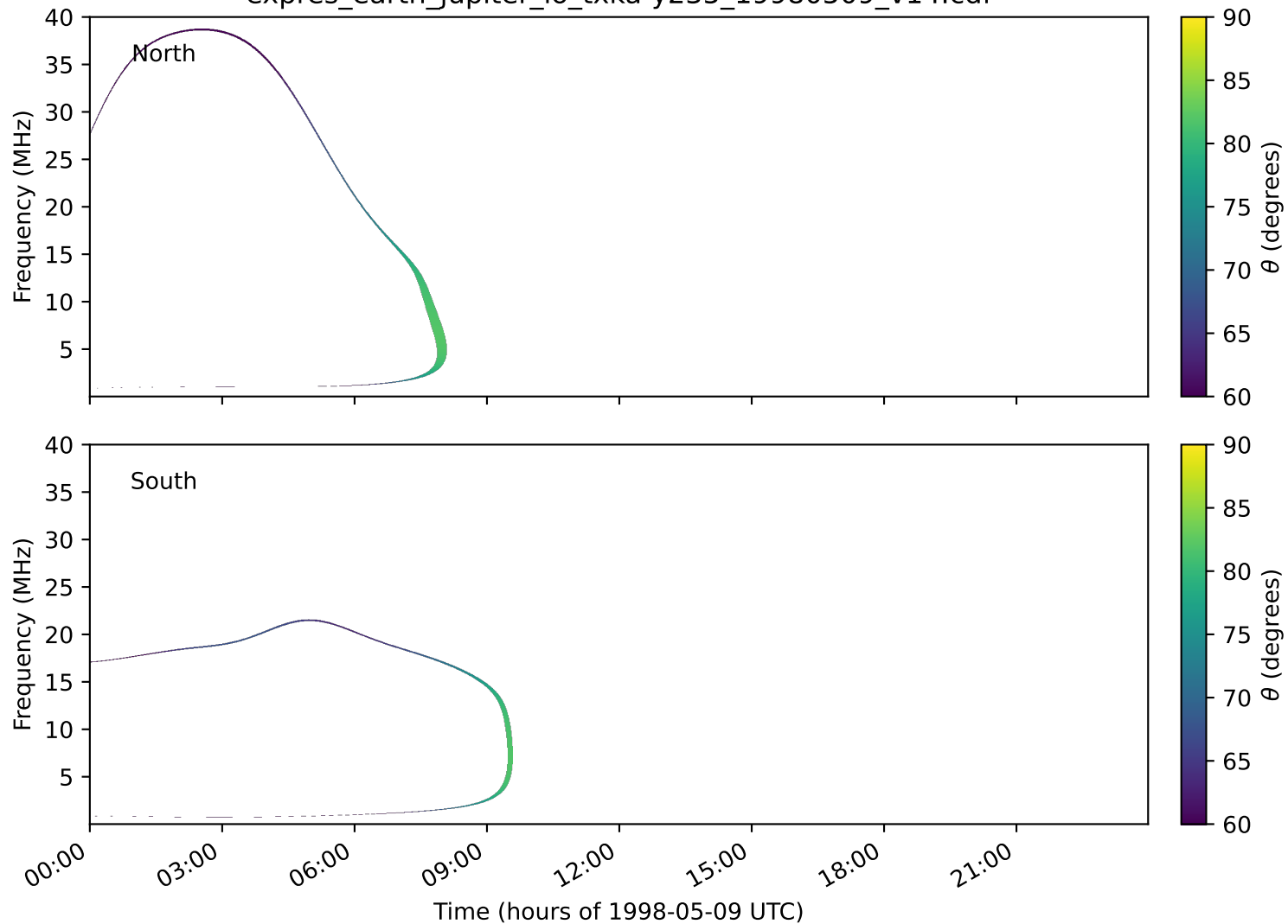
expres_earth_jupiter_io_txka-y235_19980509_v14.cdf
