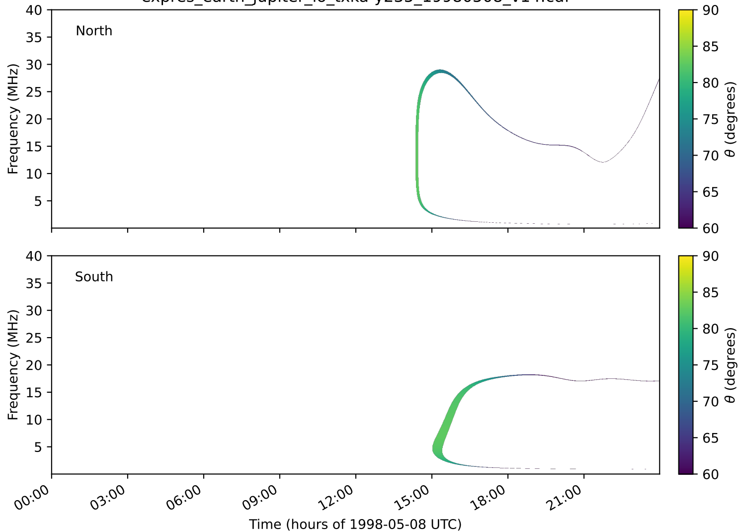
expres_earth_jupiter_io_txka-y235_19980508_v14.cdf
