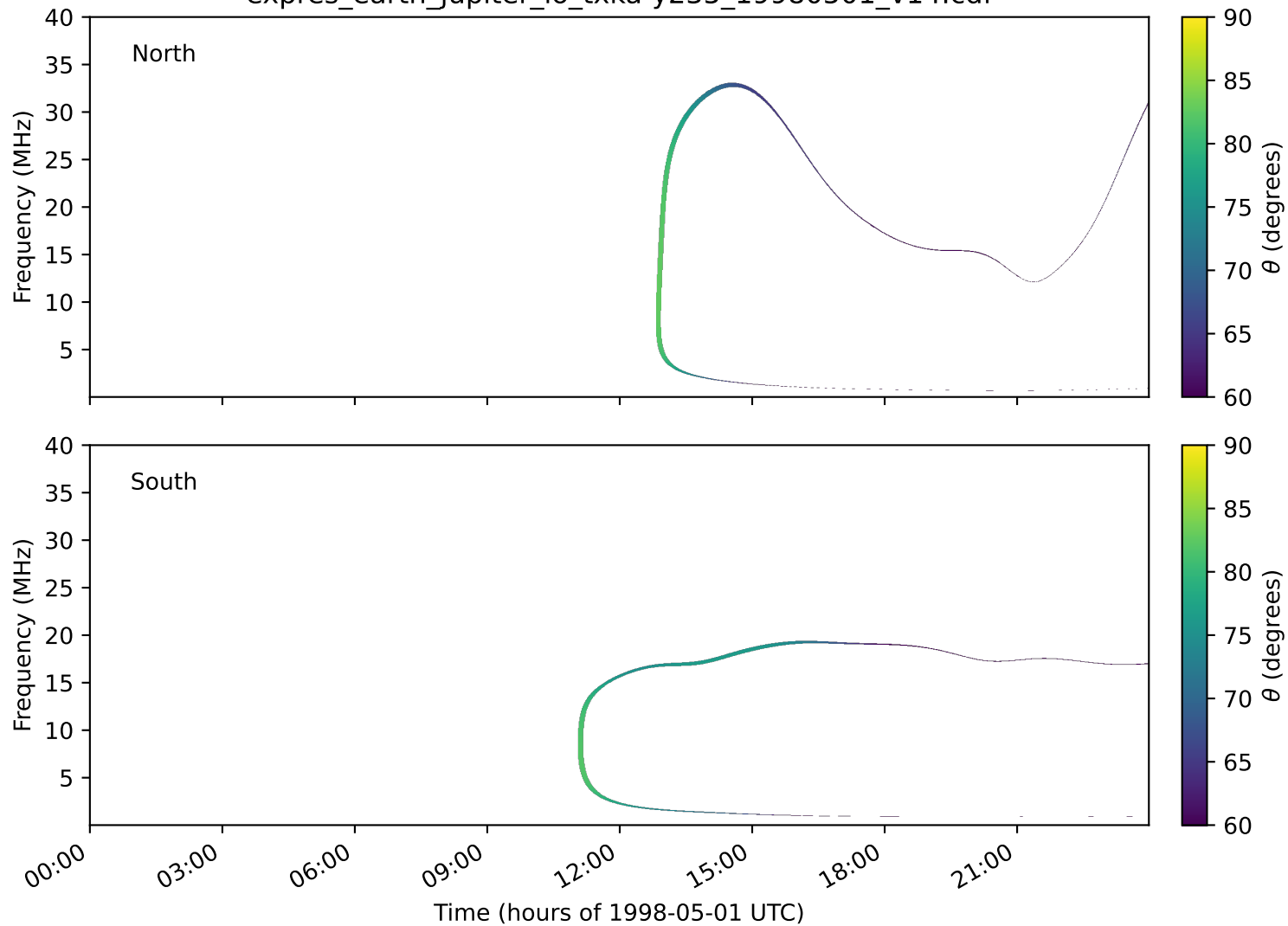
expres_earth_jupiter_io_txka-y235_19980501_v14.cdf
