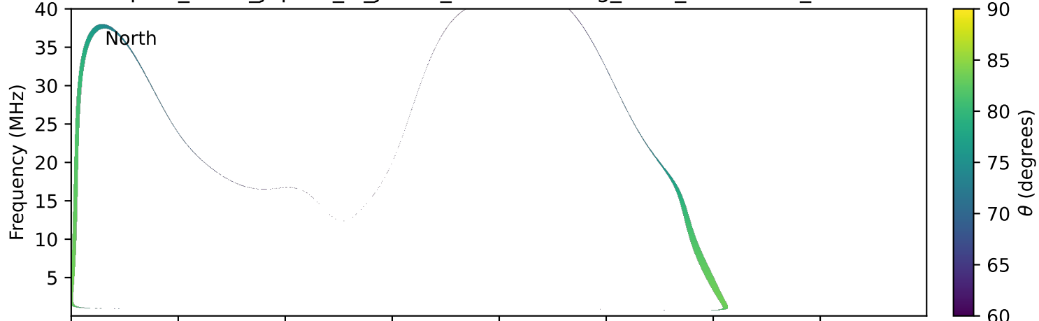
expres_earth_jupiter_io_jrm33_lossc-wid1deg_3kev_19980521_v11.cdf
